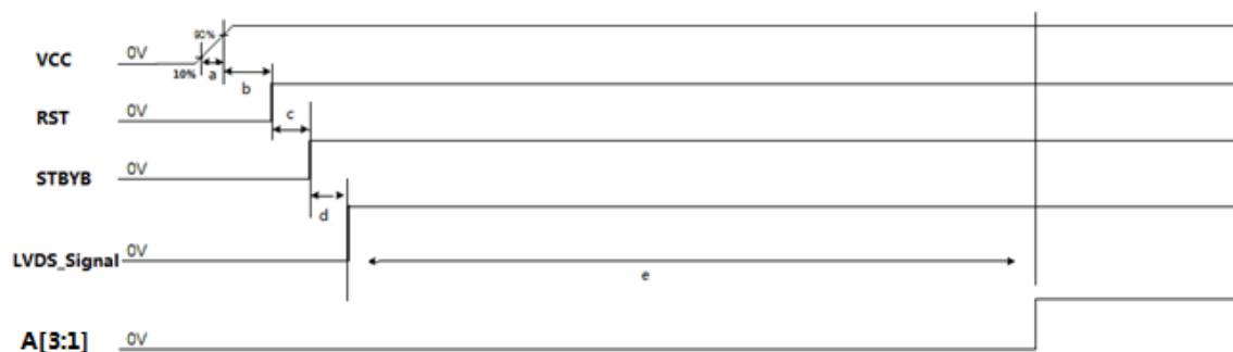
Figure 5.3.1 Power ON Sequence
