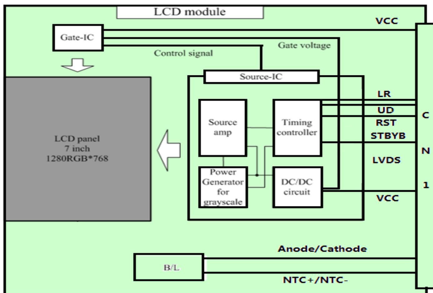
Figure 5.5.1 LCD Module Block Diagram
