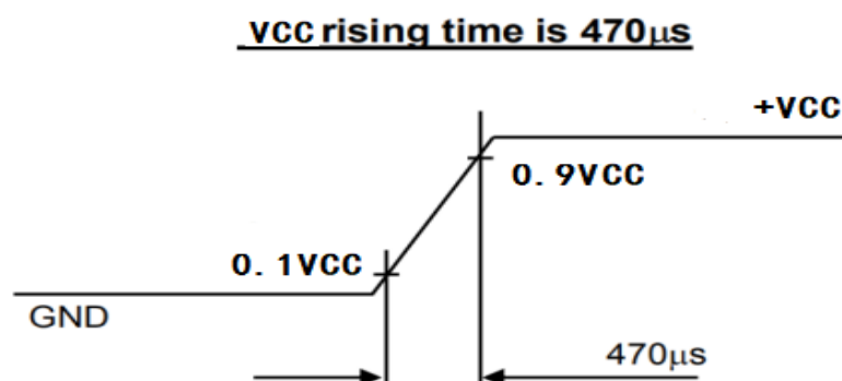
Figure5.1.3 VCC rising timing
