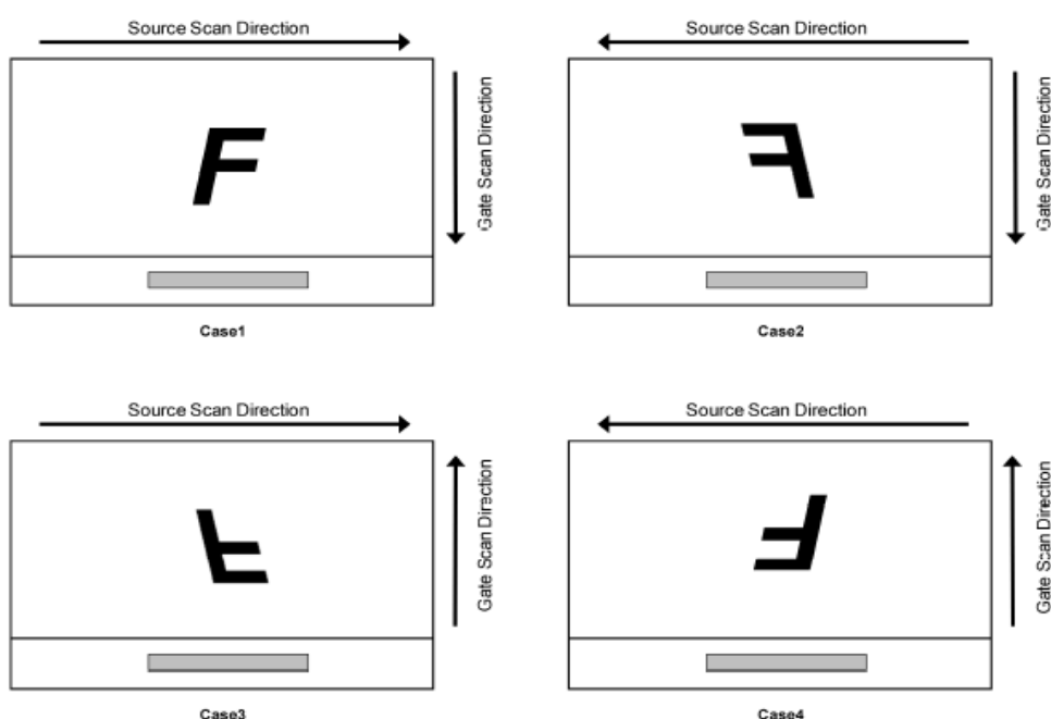
Figure3.1.1 Description of Scan Direction
