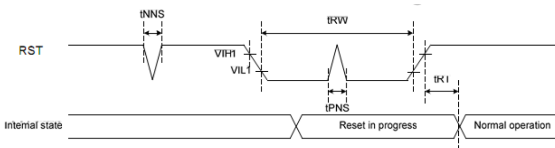
Figure 5.4.1 Reset Timing
