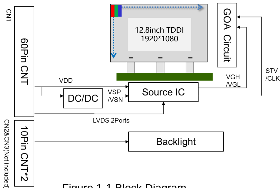
Figure 1-1 Block Diagram
