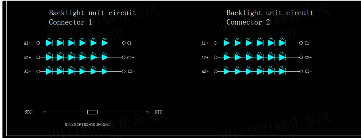
Figure 3-2 LED&NTC Diagram
