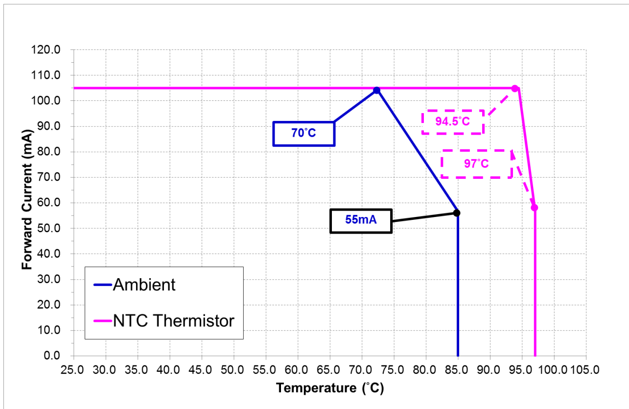
Figure 4-4 De-rating Curve
