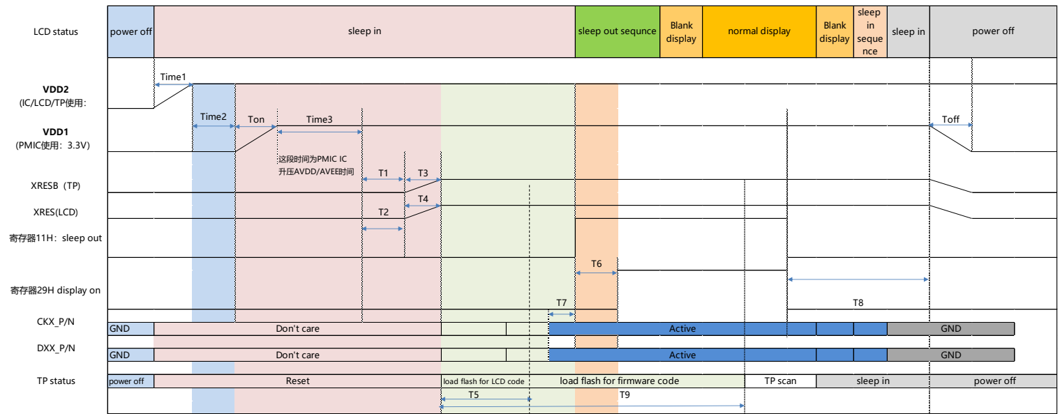
Figure 3-4 Power on/off sequence
