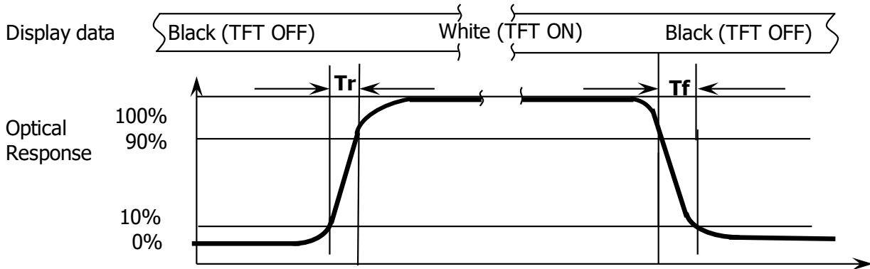
Figure 4-3 Response Time Testing
