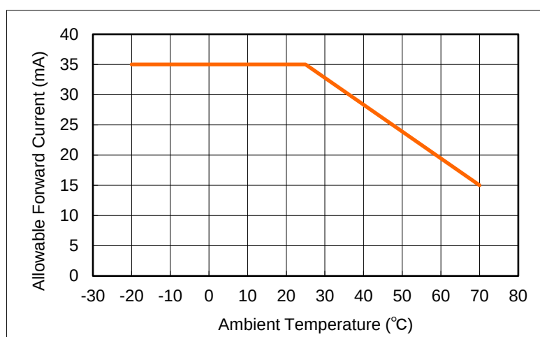
Fig. 2: Allowable Forward Current
