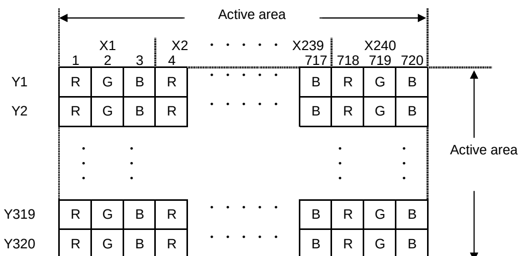
Fig. 1 Dot arrangement (FPC cable placed leftside)
