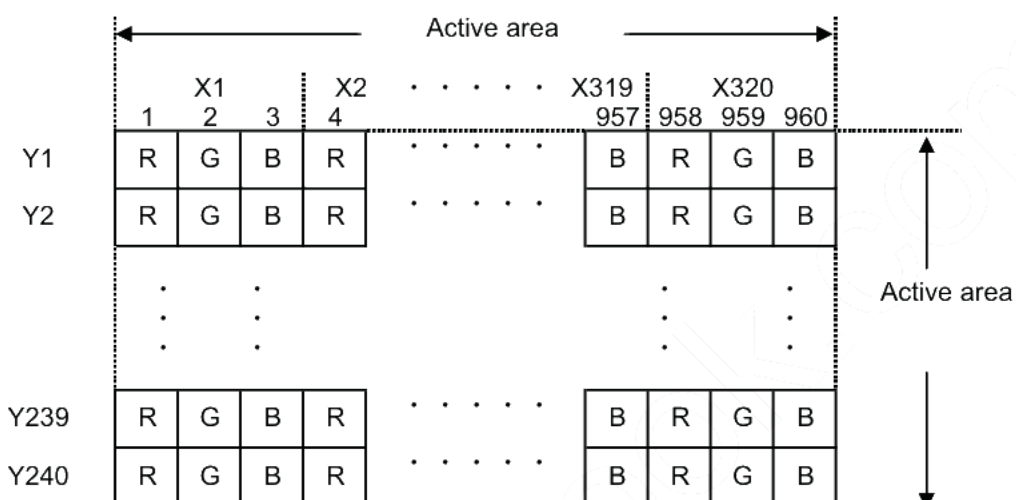
Fig. 1: Dot arrangement (FPC cable placed down)
