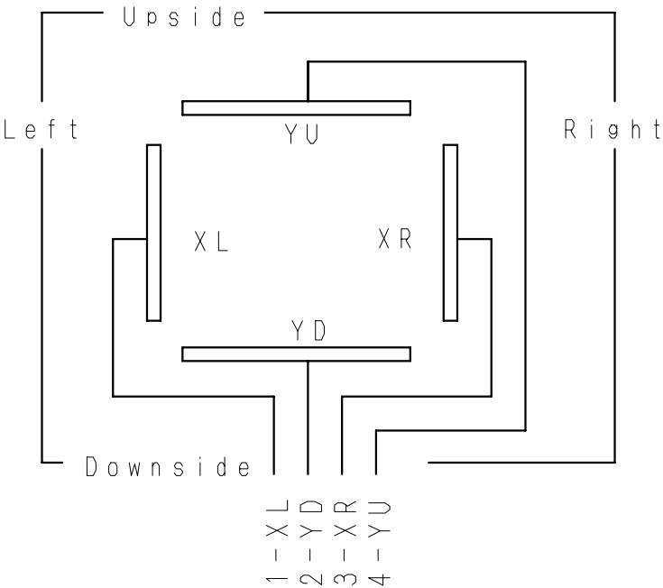
Circuit diagram
