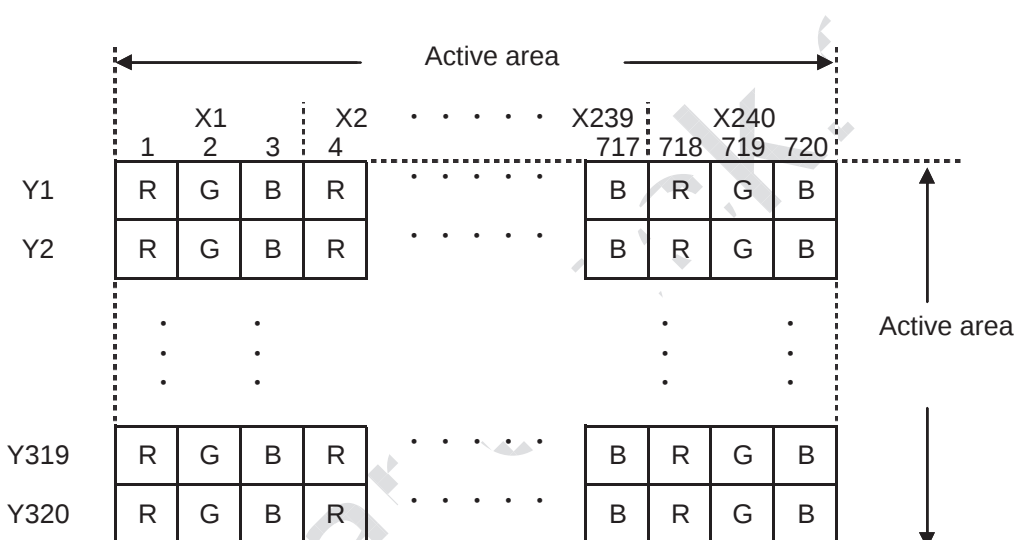
Fig. 1 Dot arrangement (FPC cable placed leftside)
