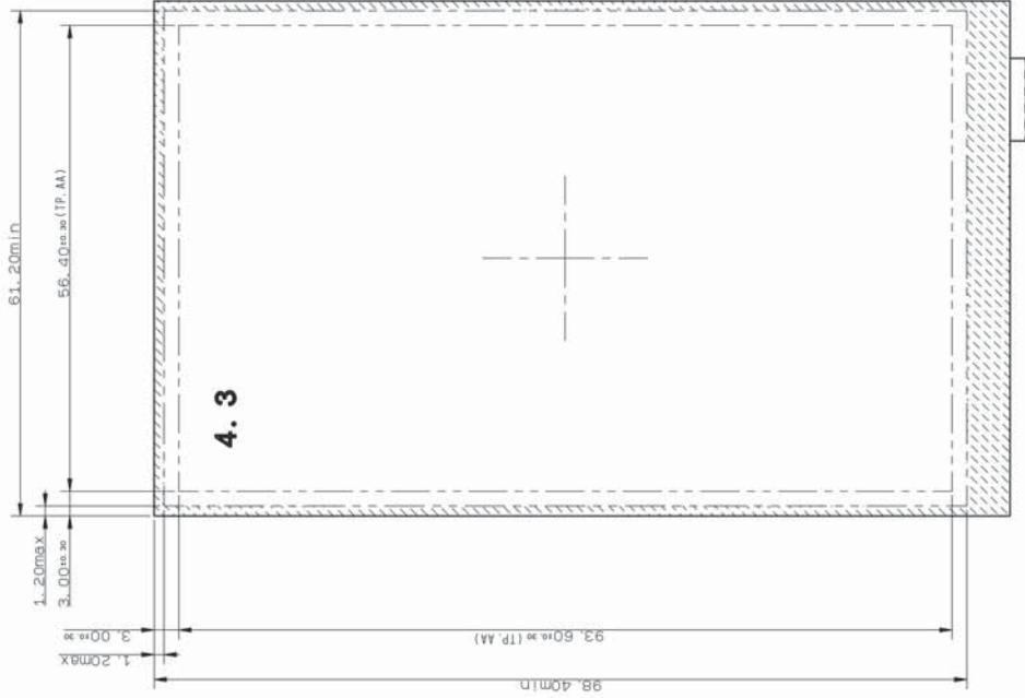
Cushion area (TOUCHPANEL)
