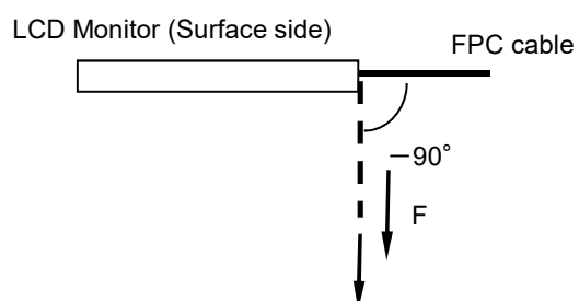
Tension Test Method for FPC cable
