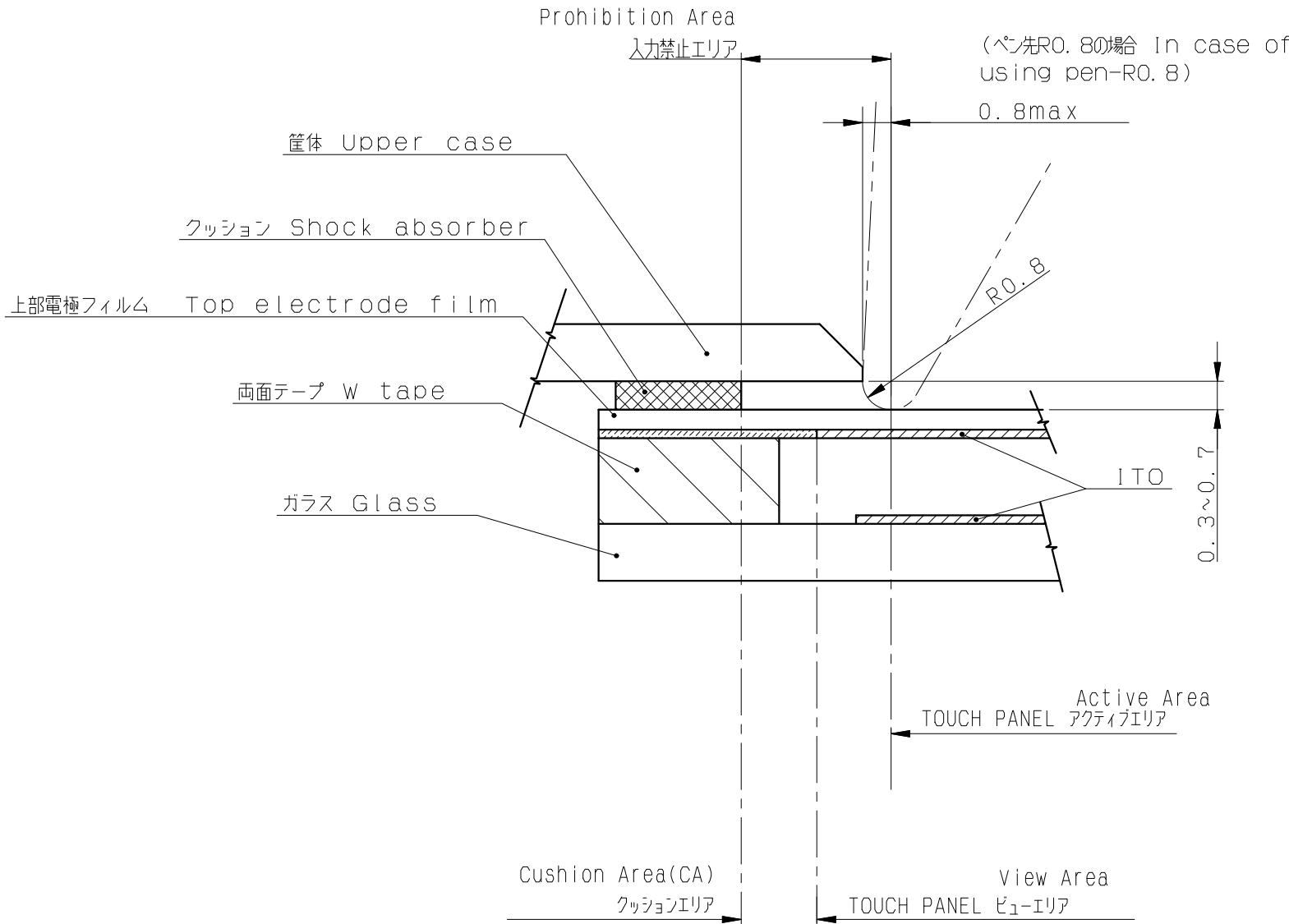
筐体設計例 Example of Housing Design (S=Free)
