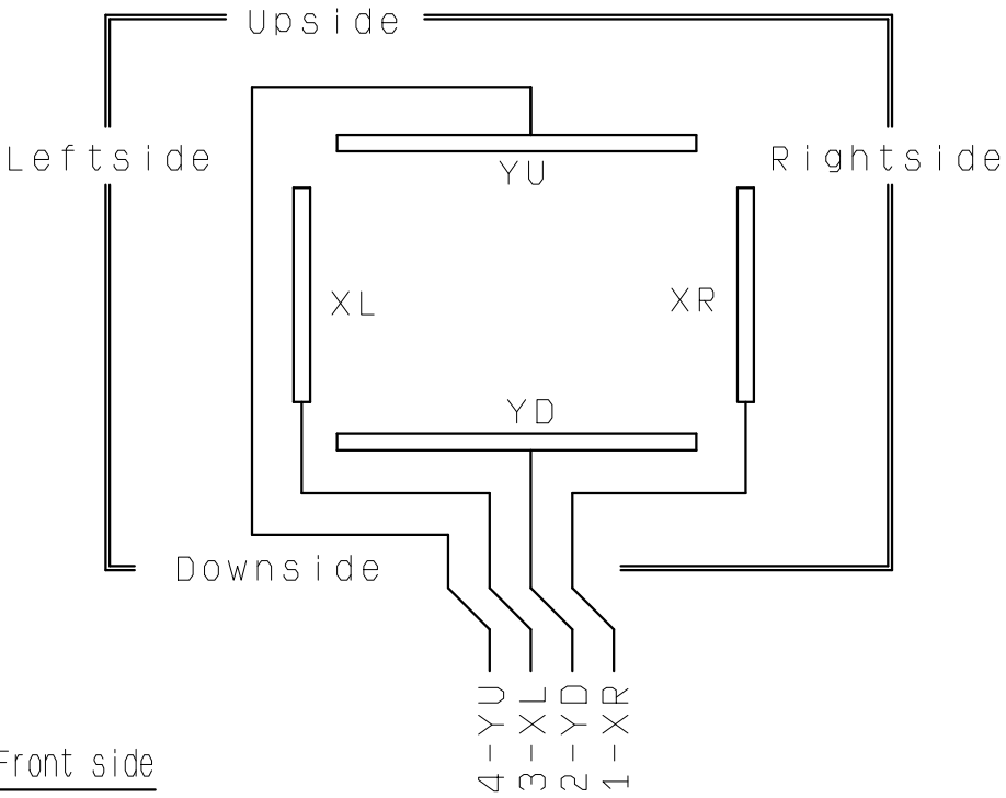
端子配列 Circuit diagram
