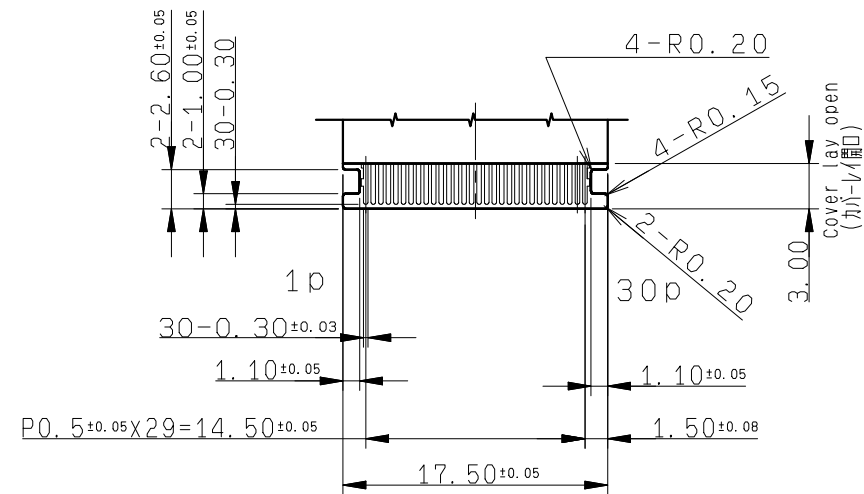
DETAIL A (S=2/1)
