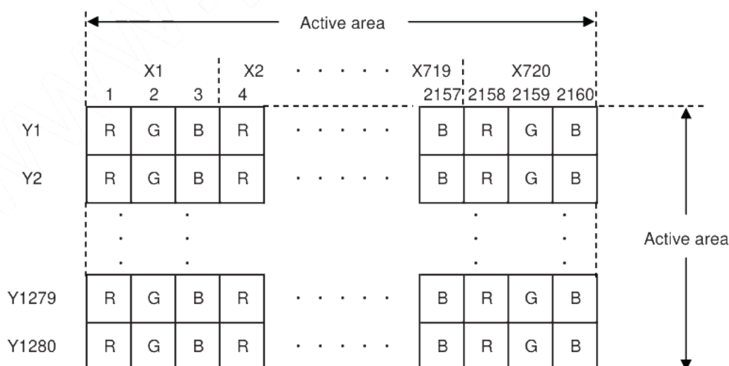
Dot arrangement (FPC cable placed)
