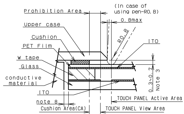
Note 7 Example of Housing Design (S=Free)
