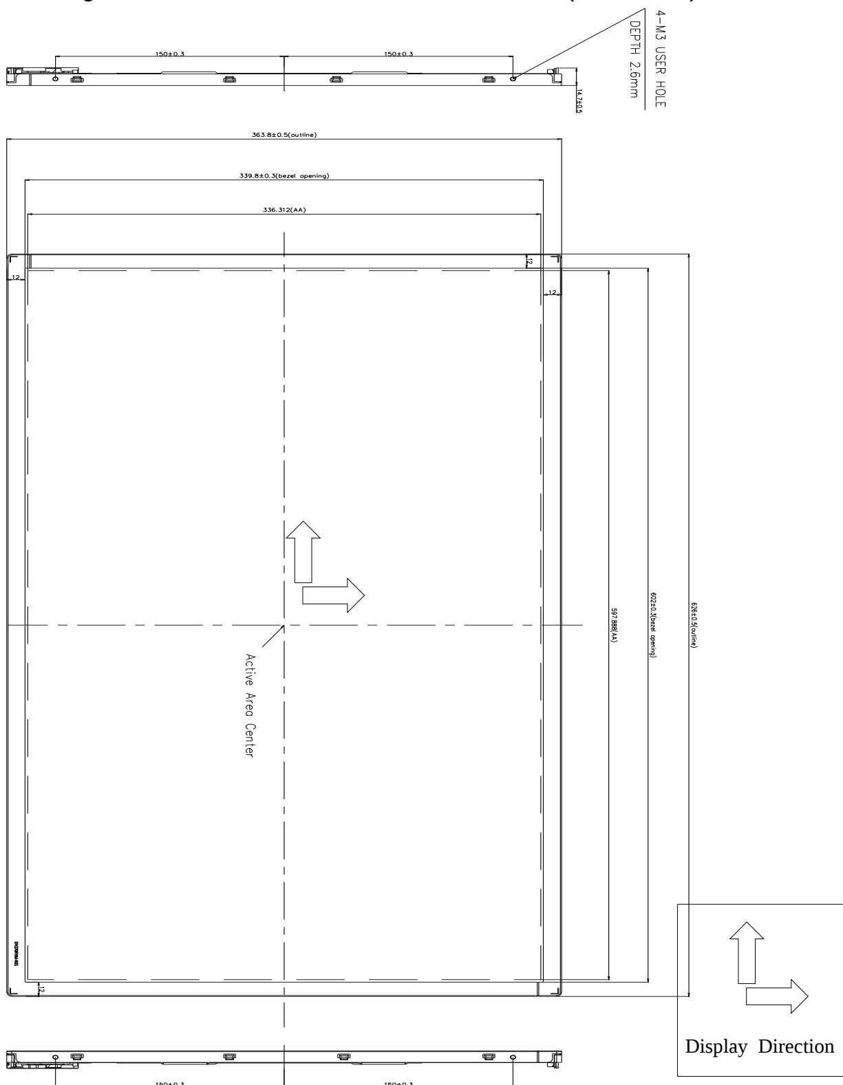
&lt; Figure 3.TFT-LCD Module Outline Dimensions (Front View) &gt;
