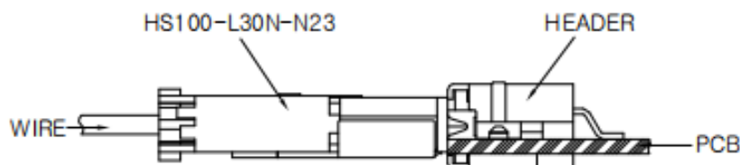
MATED CONDITION
