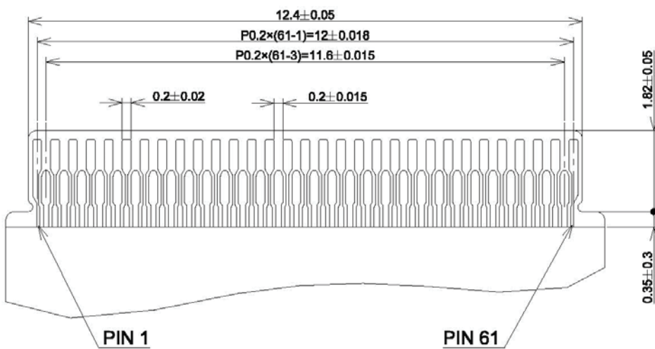
Electrode(enlarged)
