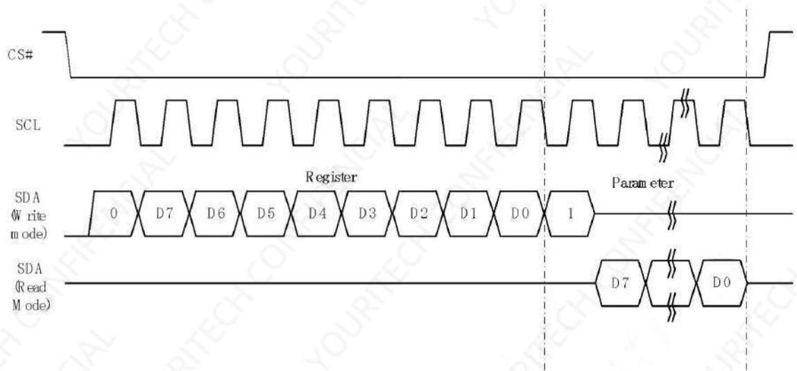
Figure 6-4: Read procedure in 3-wire SPI mode
