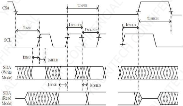
Figure 7-5: SPI timing diagram
