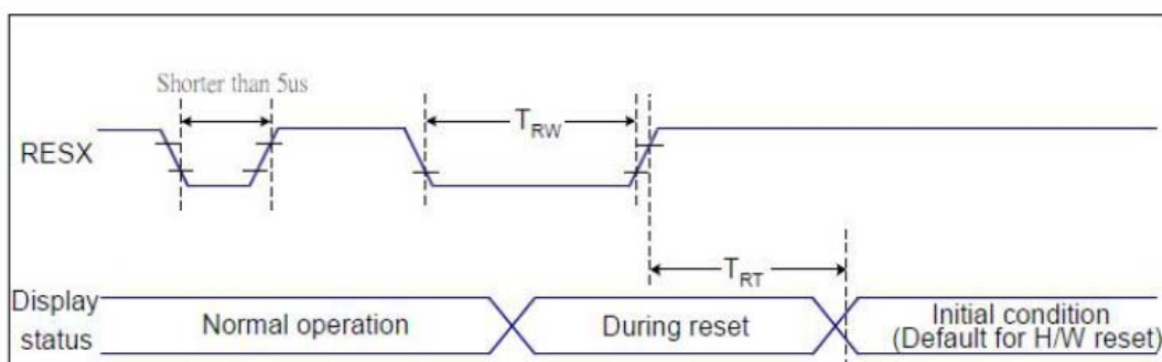
Figure 7 Reset Timing
