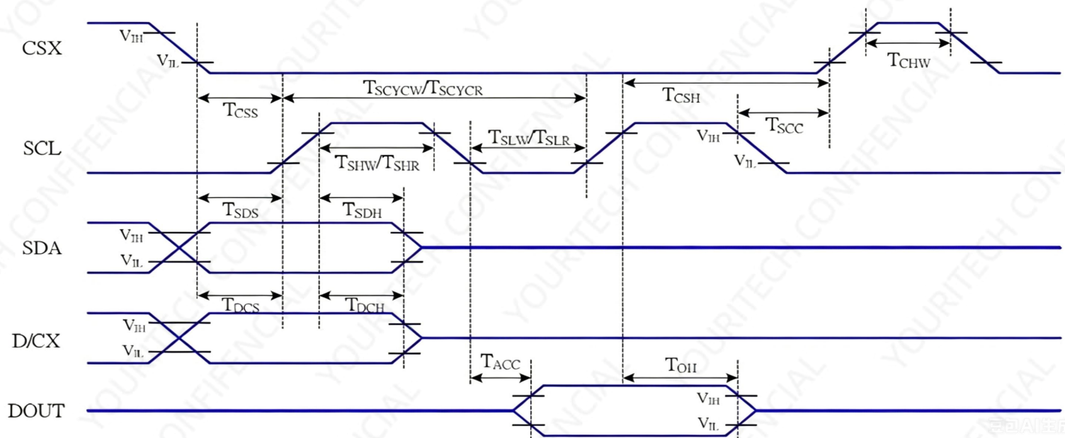
Figure6-3-1 4-line serial Interface Timing Characteristics
