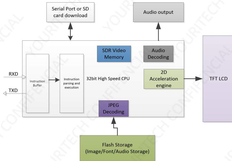
Figure 11-1 M series serial port screen internal structure diagram
