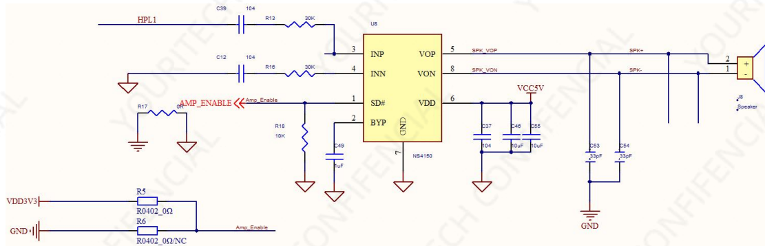
Figure 6-2: Audio reference circuit
