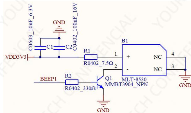
Figure 6-3 Buzzer reference circuit
