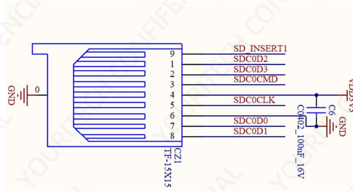
Figure 6-1 SD deck circuit schematic
