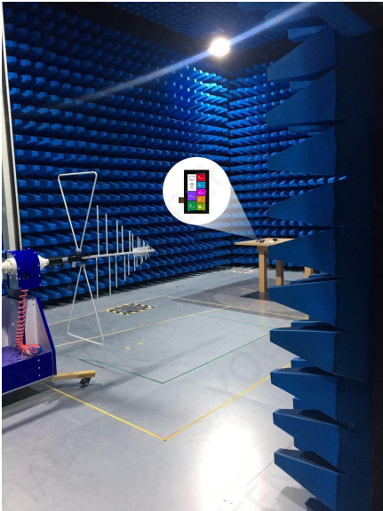
Figure 7-5 Radiation test chart
