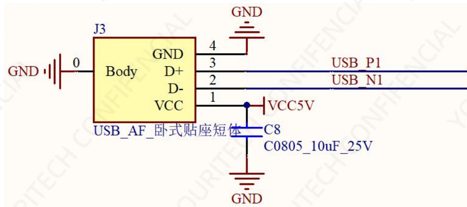
Figure 6-4 USB flash drive reference circuit
