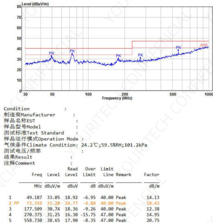
Figure 7-7 Radiation test vertical
