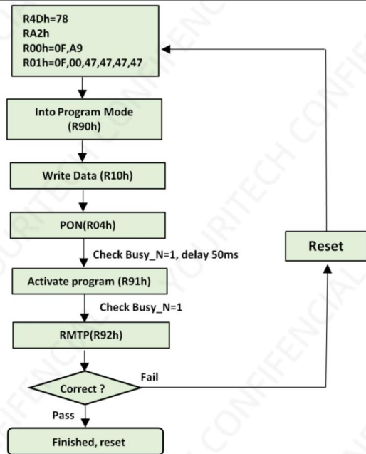
The sequence of programming MTP(Internal power)
