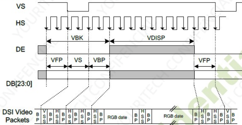
Figure. 10.11 Vertical Timings for DSI Video mode I/F
