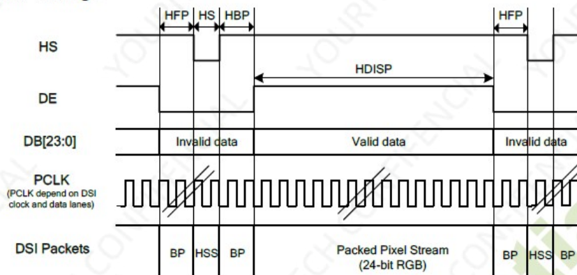
Figure. 10.13 Horizontal Timing for DSI Video mode I/F
