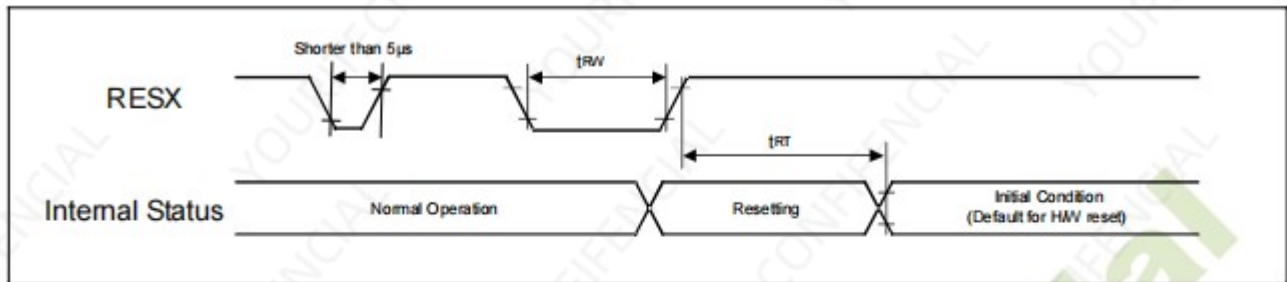
Figure. 10.5 Reset input timings
