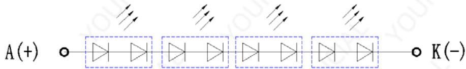
BLU CIRCUIT DIAGRAM
