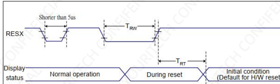
Figure 9 Reset Timing
