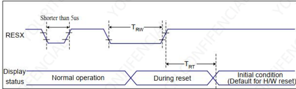
Figure 9 Reset Timing
