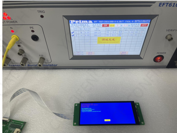
Figure 5-4 Group pulse test diagram
