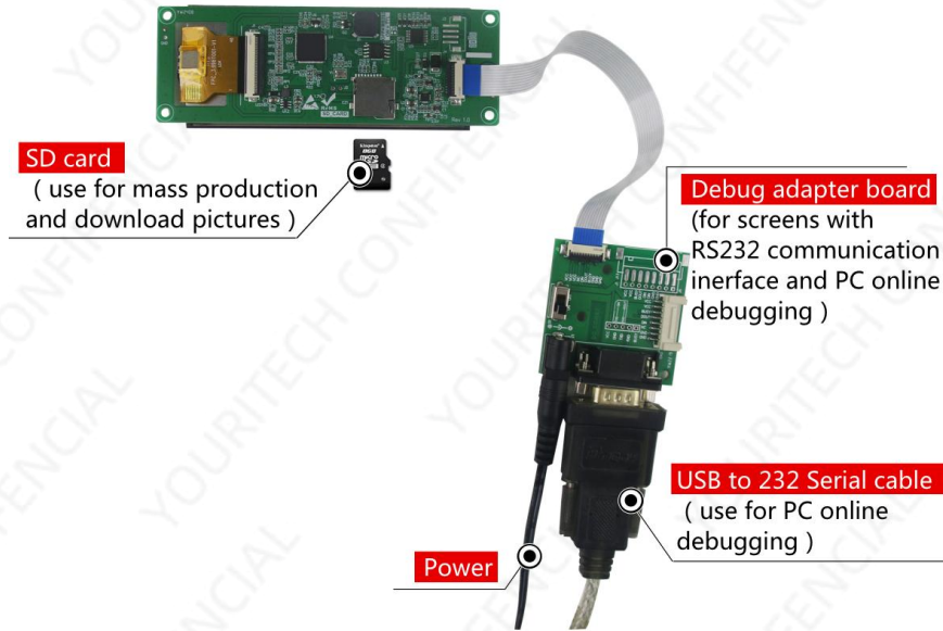
Figure 1-3 Debugging tool diagram
