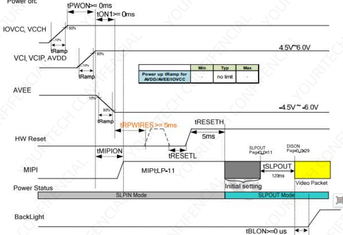
Figure 9.10: Power on sequence for differential power mode
