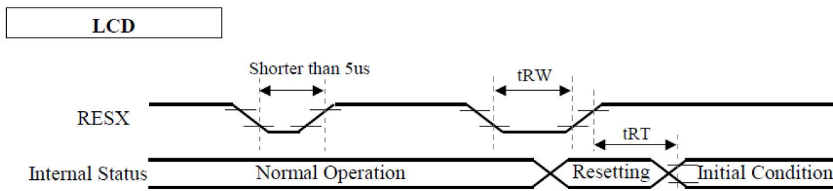
Fig.8.4.1 RESX Operation
