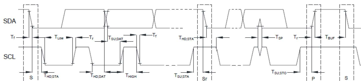
Figure 8.7.1 I2C timing
