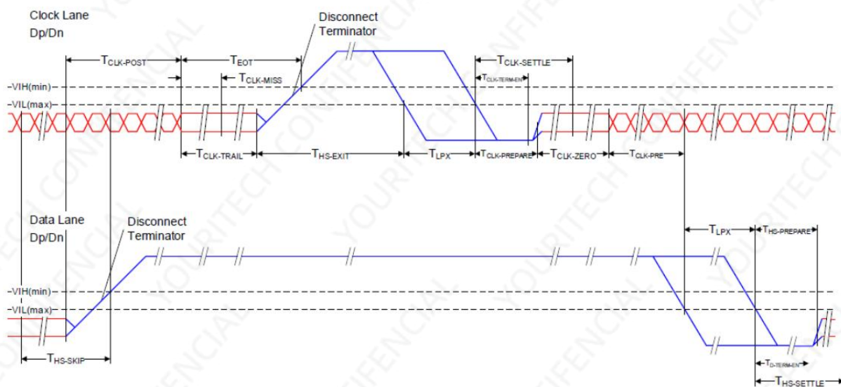
Figure 8-4-2-2 HS Clock Transmission
