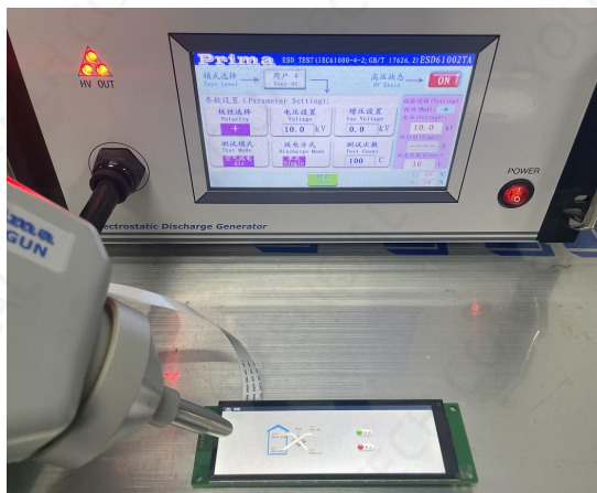
Figure 5-2 ESD test diagram
