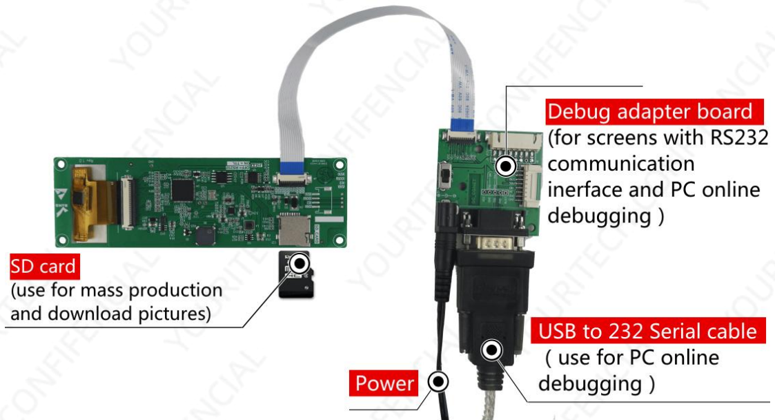
Figure 1-3 Debugging tool diagram
