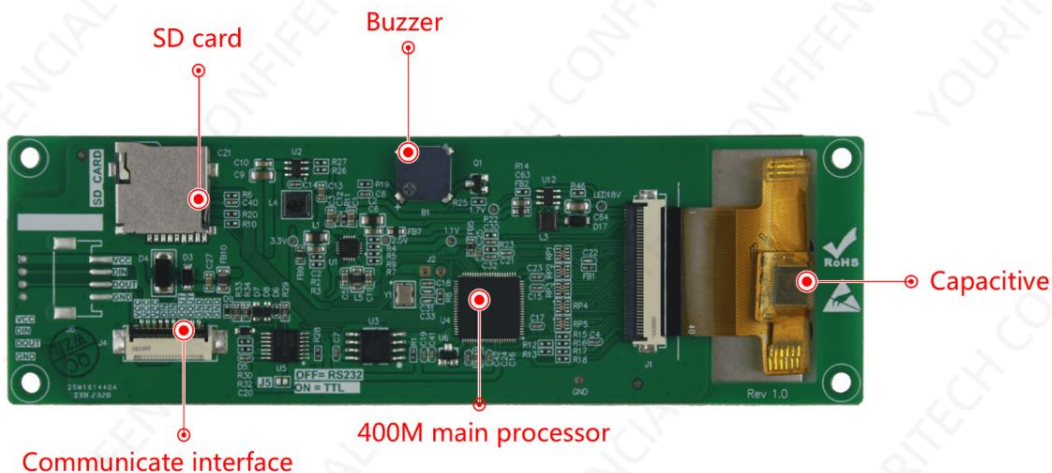
Figure 1-2 Hardware configuration diagram
