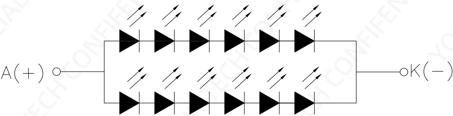
LED (B/L) CIRCUIT
