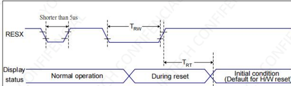
Figure 9 Reset Timing
