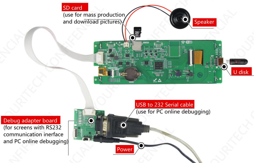
Figure 1-3 RS232 debugging tool Diagram
