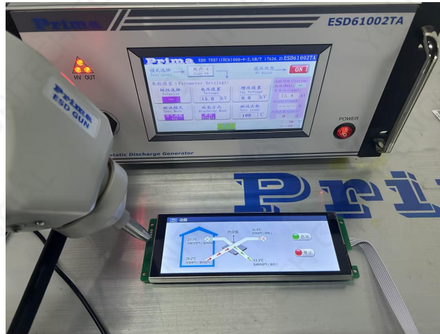
Figure 5-2 ESD Test
