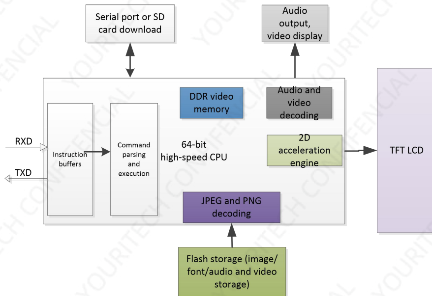
Figure 2-1 Internal structure diagram of DH series serial port screen
