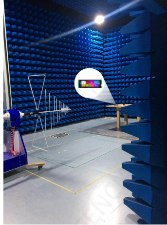
Figure 5-5 Radiation test chart
