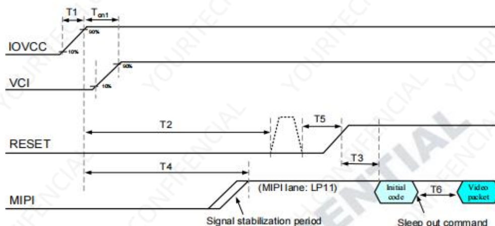
Figure 1 Power on sequence at PCCS[1:0]=[1,0] mode
