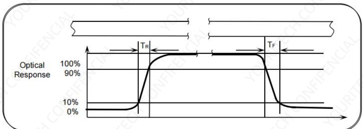
Figure2 Response Time Testing
