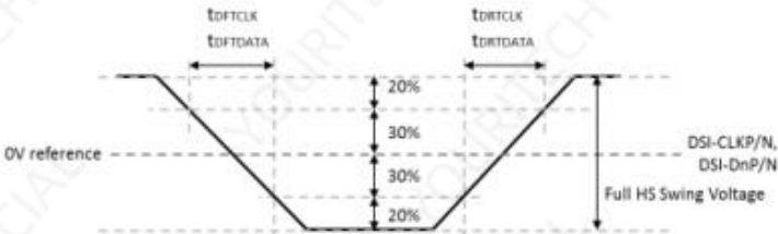
Figure 4-7 Rsing and Falling Timings
