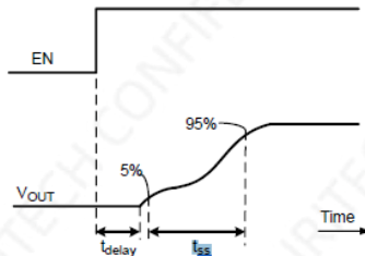
Figure 20. Soft-Start Waveform
