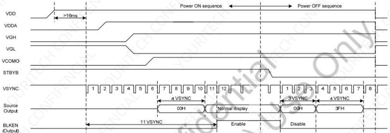
Power-On/Off Timing Sequence:
