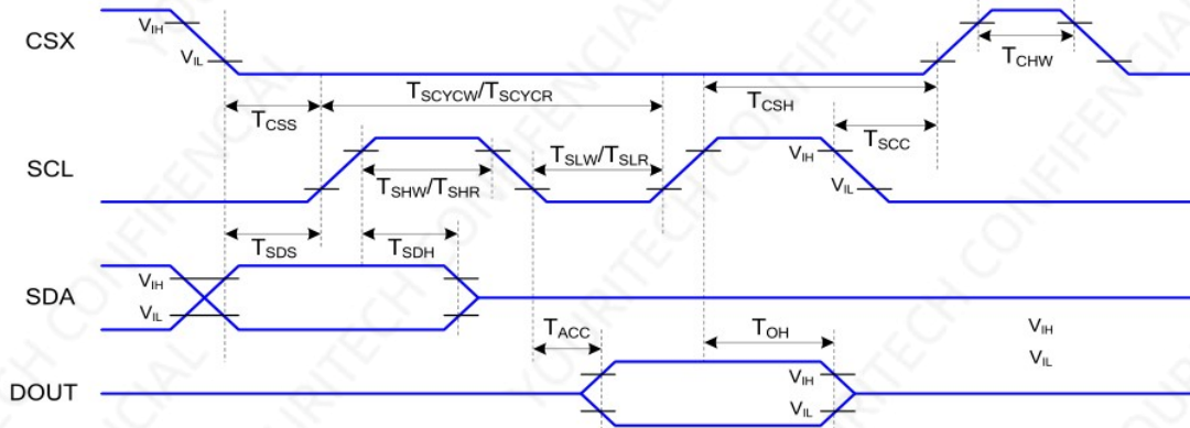
Figure 5.1 3-line serial Interface Timing Characteristics
