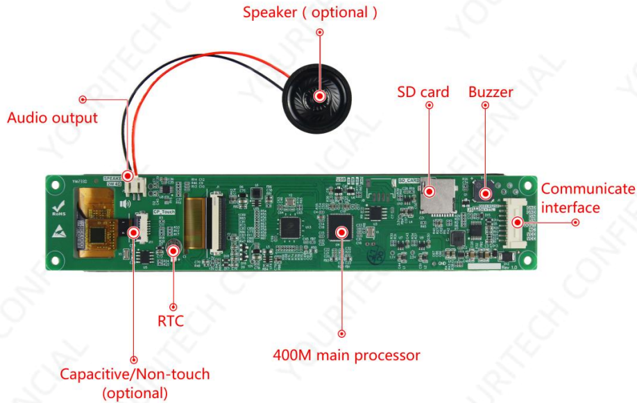
Figure 1-3 Hardware configuration diagram
