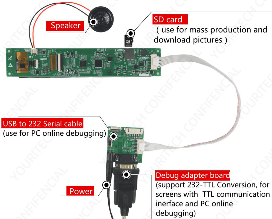
Figure 1-4 Debugging tool diagram
