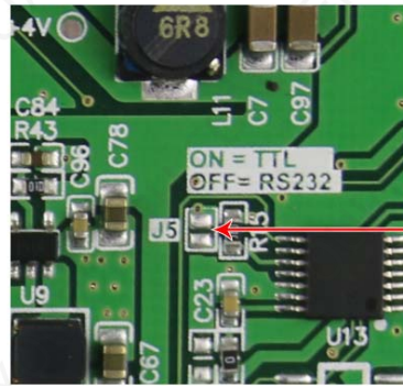
Diagram 5- 1 Switch RS232&TTL
