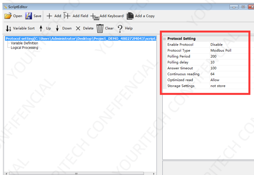
Diagram 6 - 2 Protocol configuration
