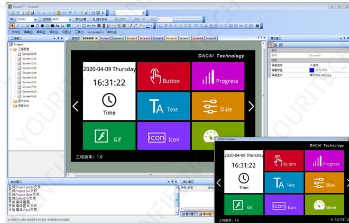
Diagram 9-1 VisualTFT Main interface
