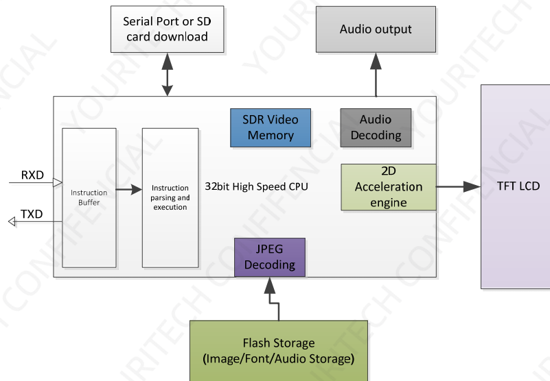
Diagram 8-1 M series product internal structure diagram of serial serial screen
