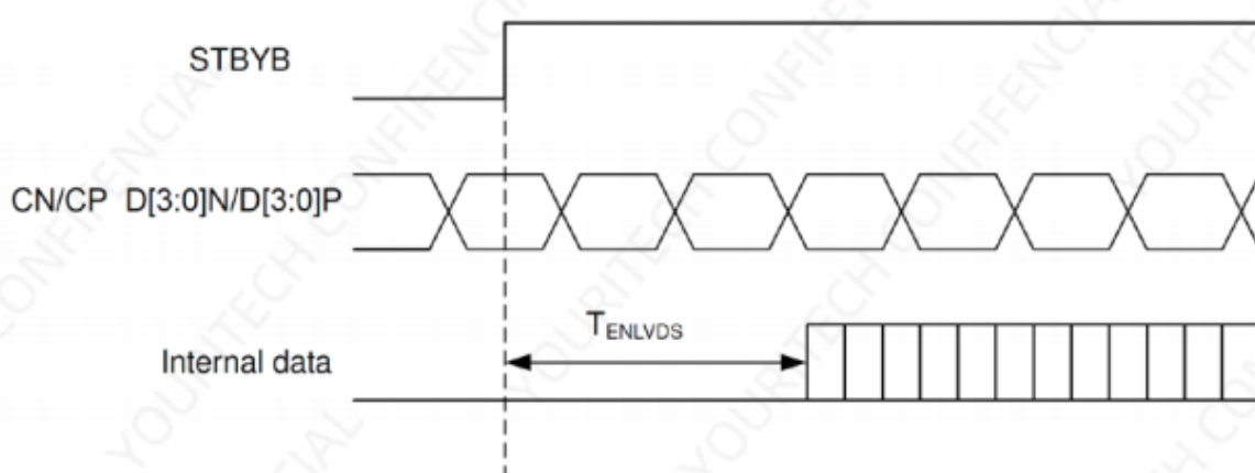
LVDS wake up time
