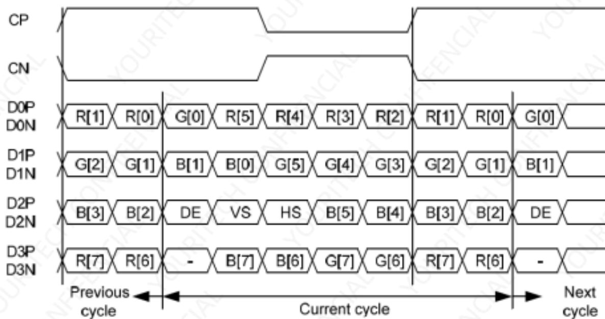
LVDS Input signal VESA format:
