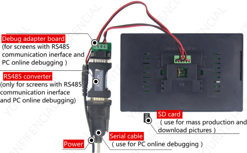
Figure 1-3 RS485 debugging tool diagram
