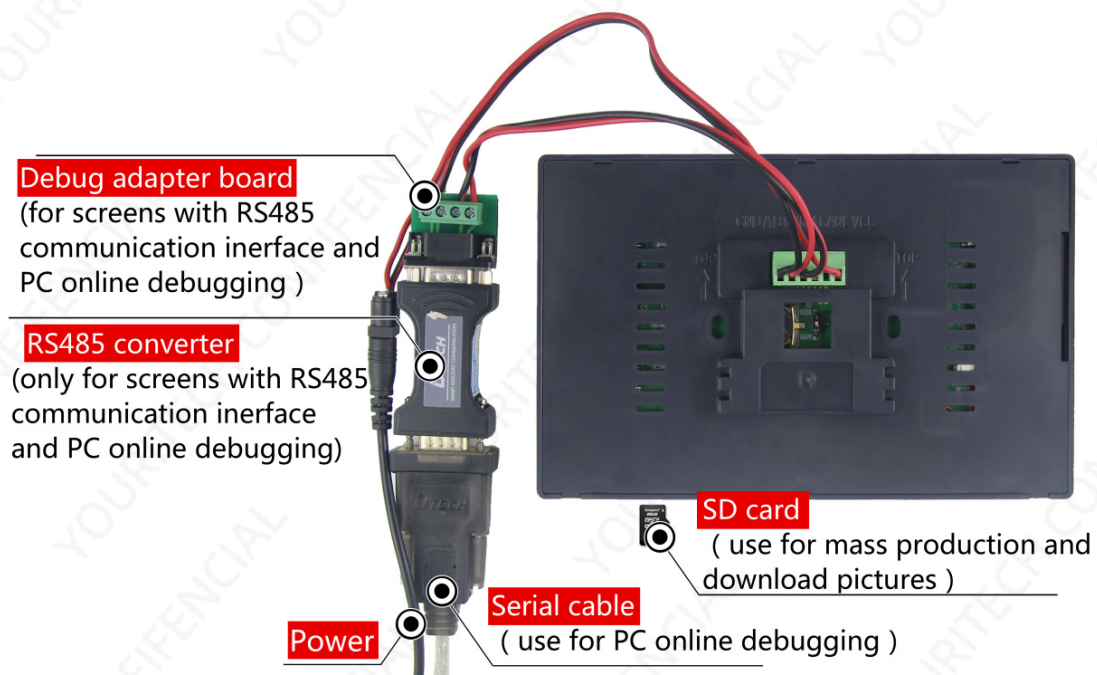
Figure 1-3 RS485 debugging tool diagram
