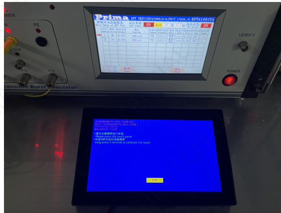
Figure 5-4 Group pulse test diagram
