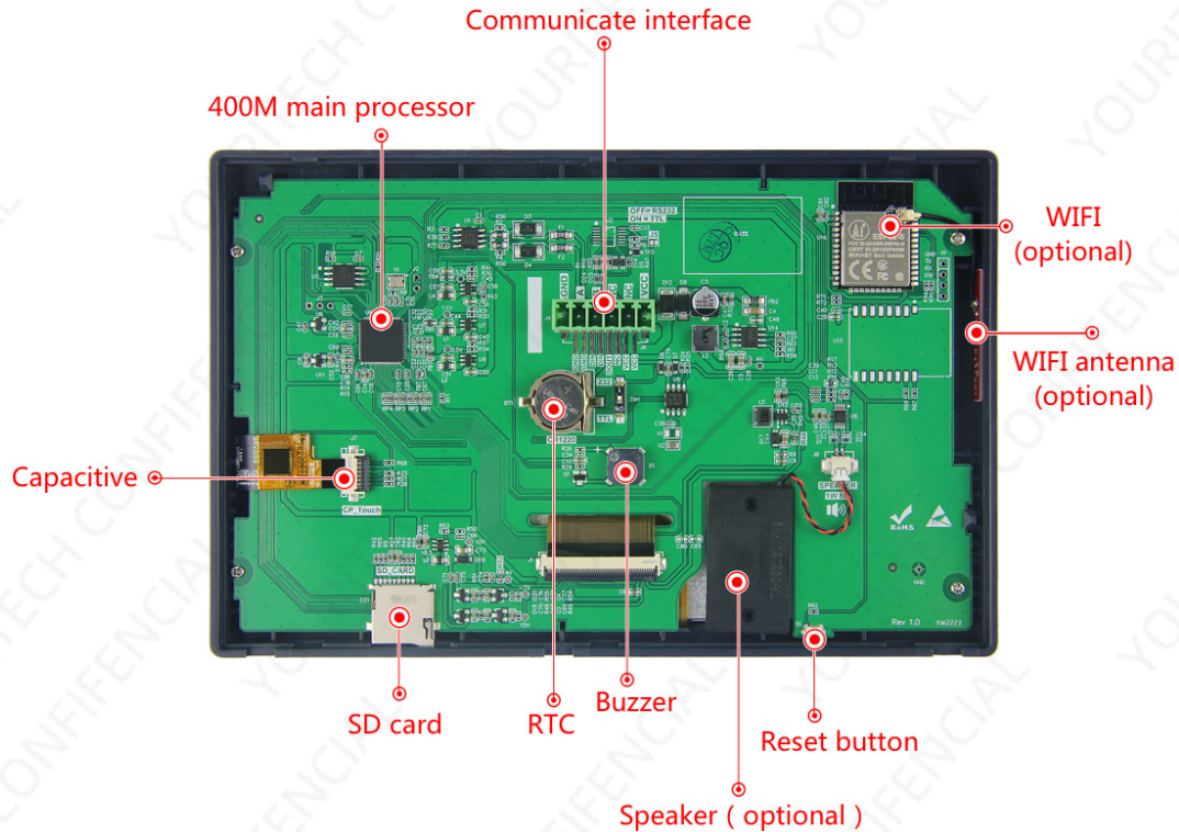
Figure 1-2 Hardware configuration diagram
