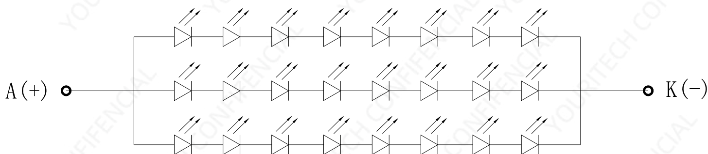
B/L Circuit
