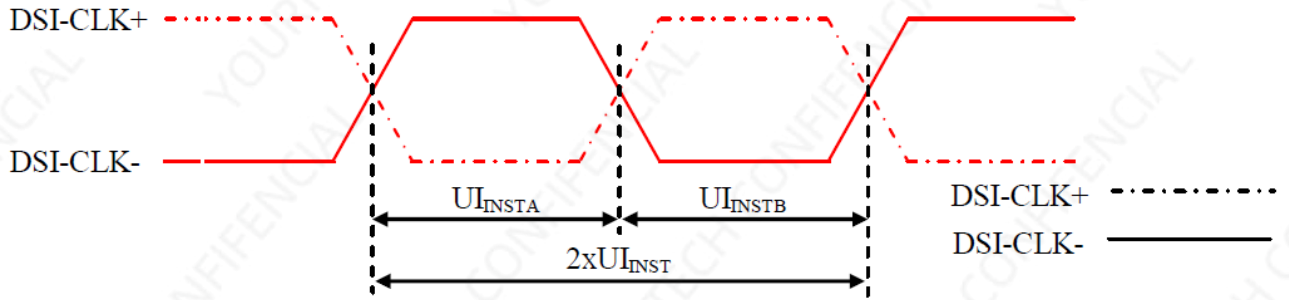
Figure 5.1.1 DSI Clock Channel Timing
