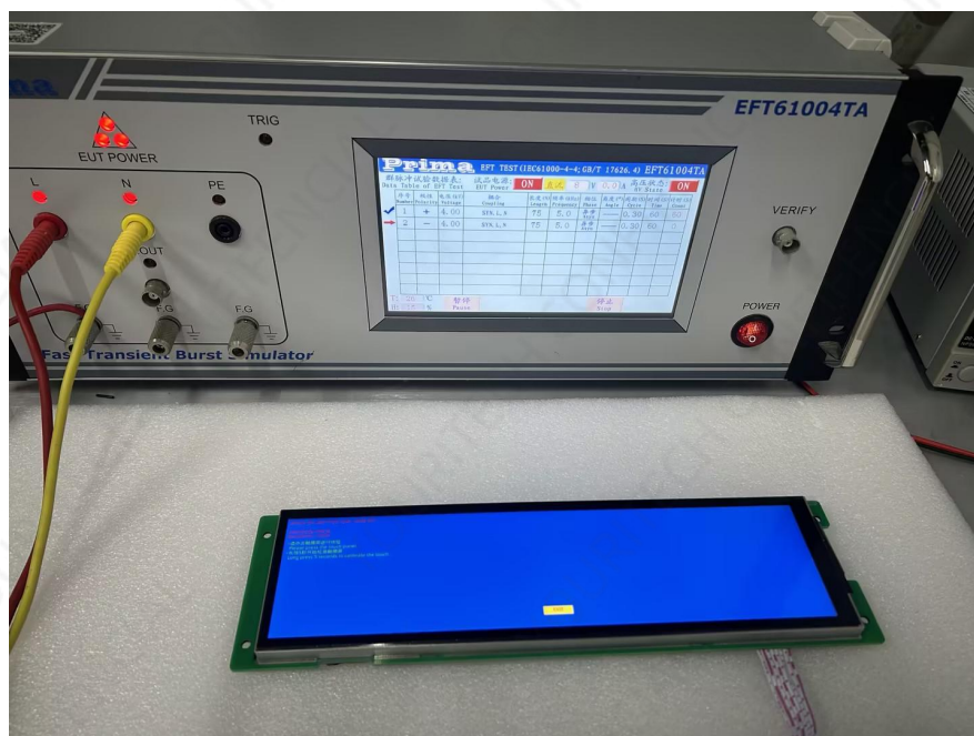
Figure 5-4 group pulse test diagram
