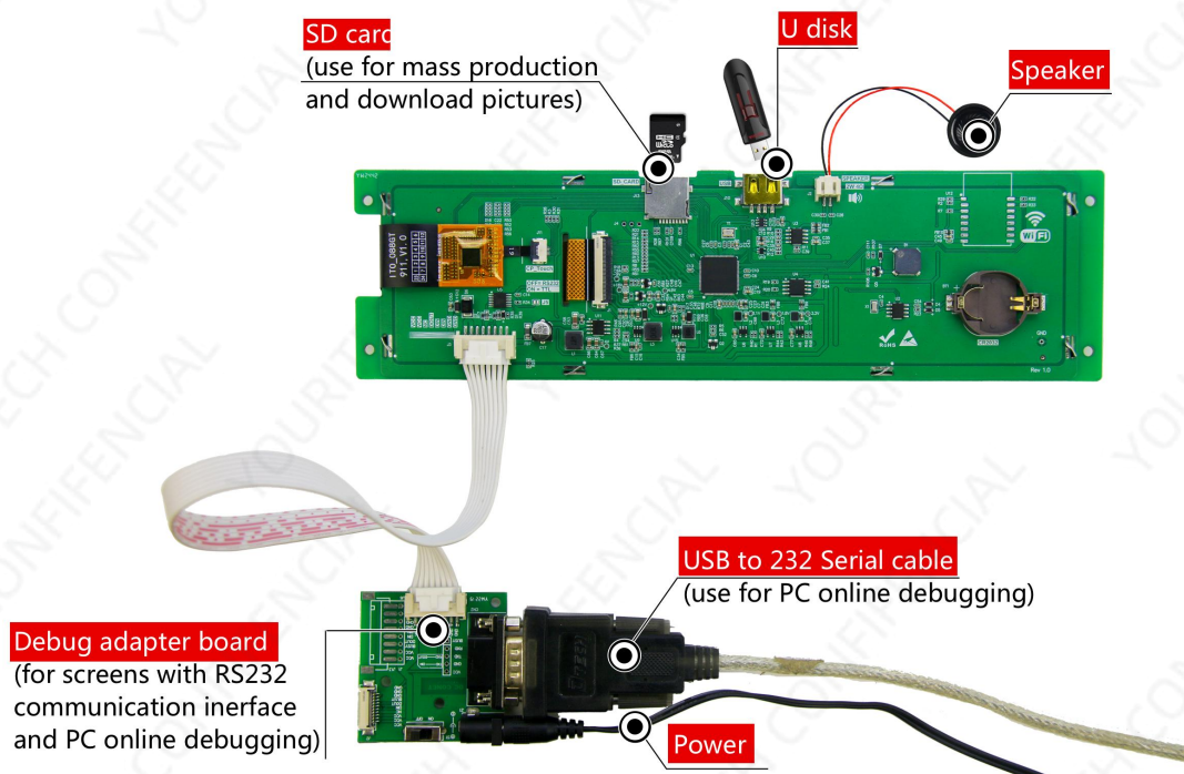
Figure 1-3: Debugging tool diagram
