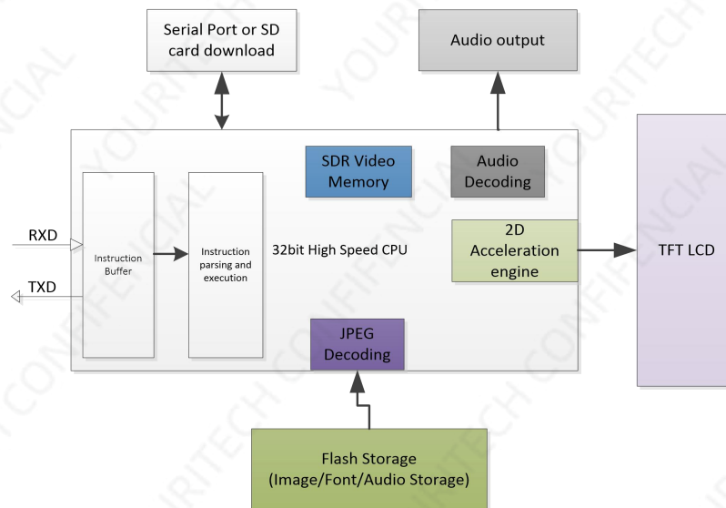
Figure 2-1 Internal structure diagram of the serial port screen of the DH series
