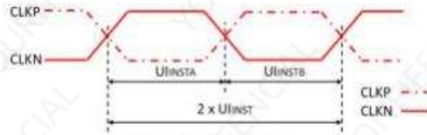
Figure 4-5 Clock Timing
