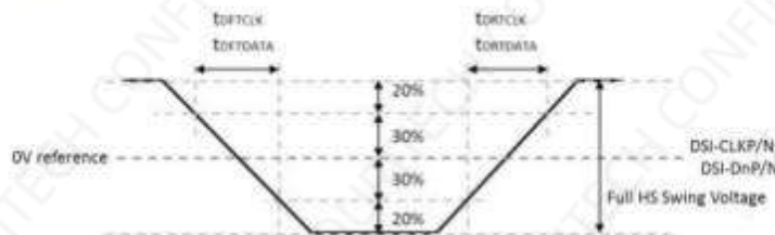
Figure 4-7 Rring and Falling Timings
