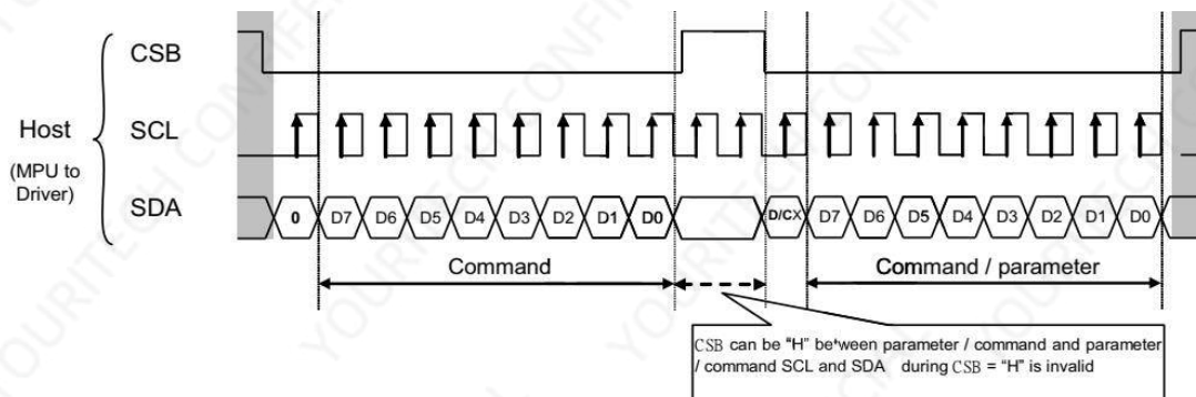
Figure 6-2: Read/Write procedure in 3-wire SPI mode
