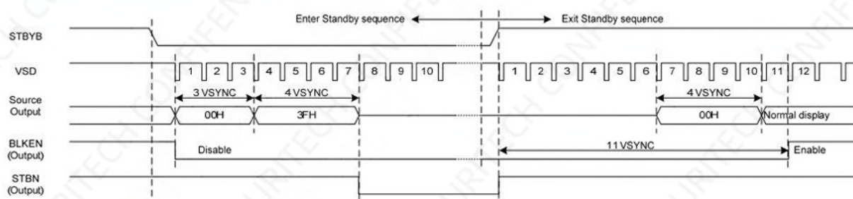
Enter and Exit Standby Mode Sequence:
