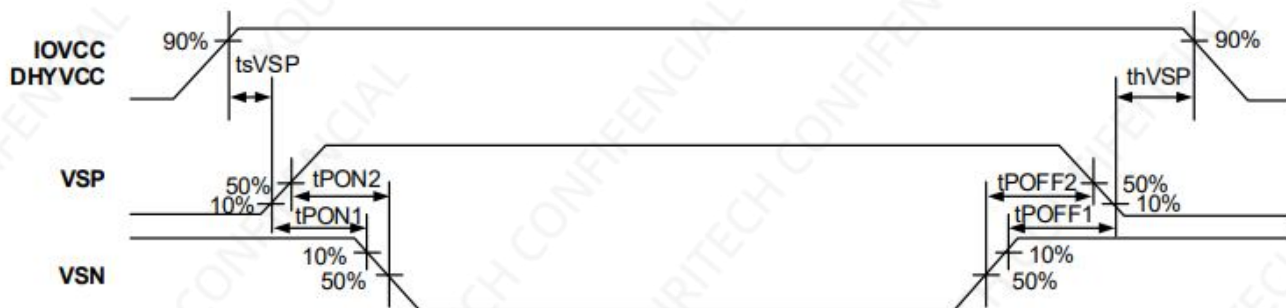
Figure 15 Power On/Off Sequence
