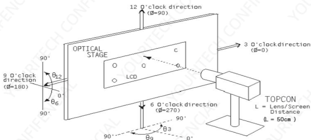
FIG.3. The definition of viewing angle 视角定义
