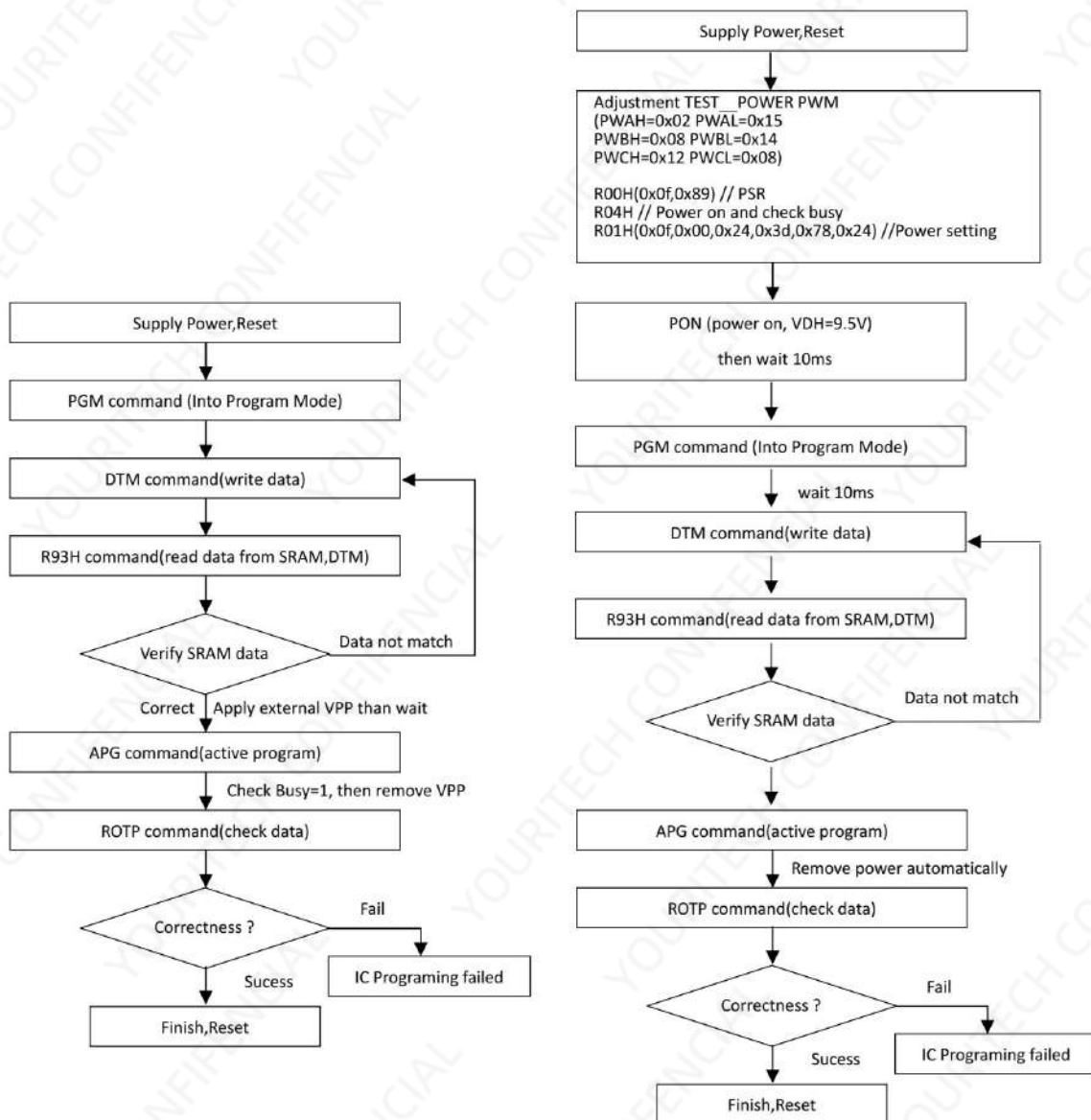
OTP Programming Flow (External VPP)
