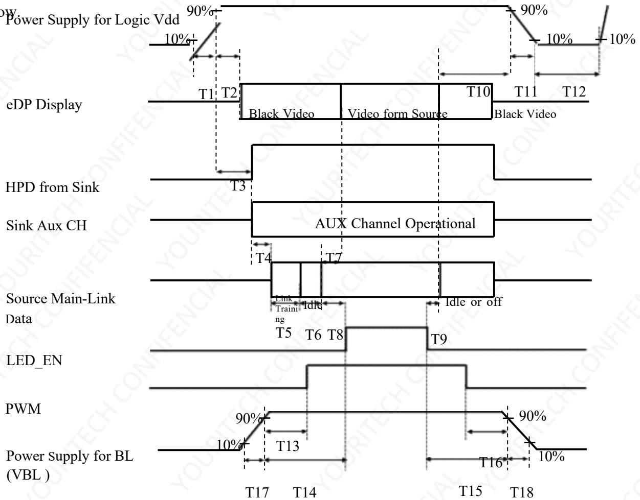
Figure 8. Power Sequence
